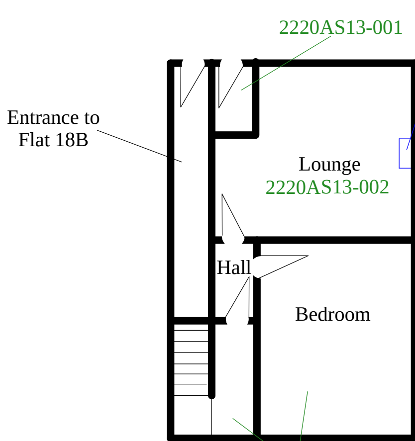
2220AS13-001 Ground floor
